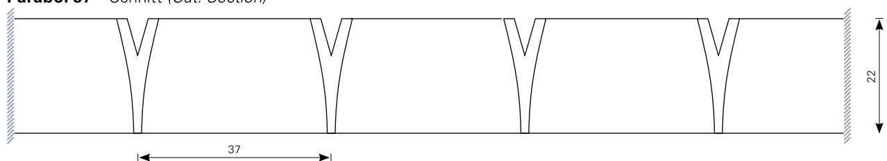
Parabol 37 – Schnitt (Cut. Section)
